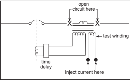
Secondary testing with test winding
