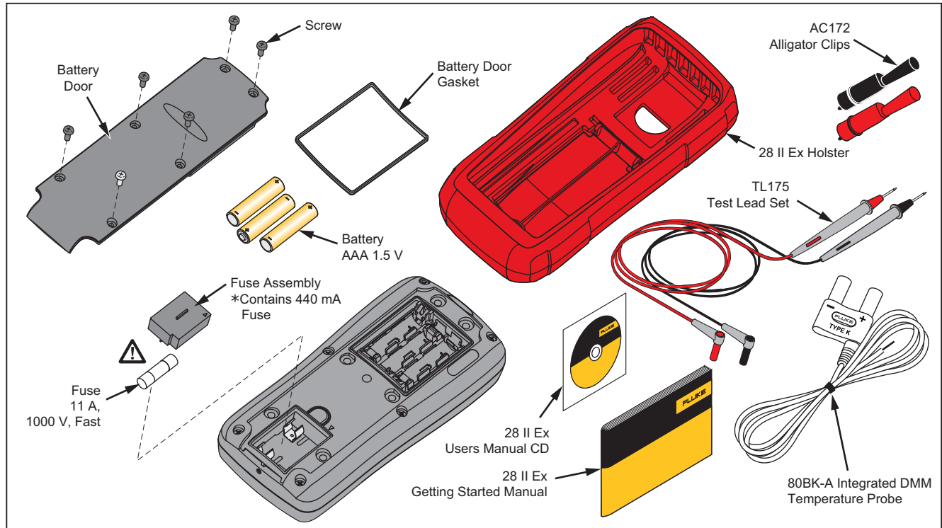
Figure 4. Replacement Parts
