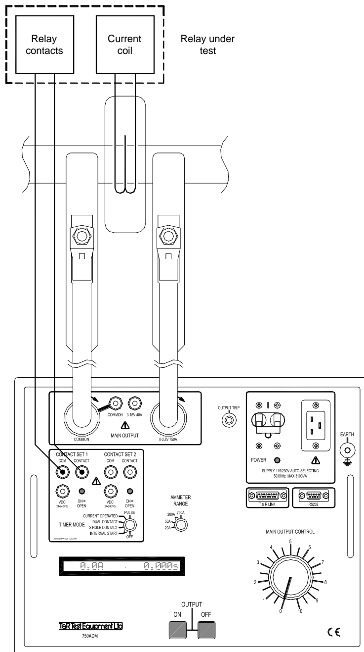
Figure 3.1 Primary injection of overcurrent relay
