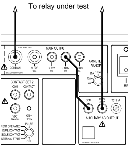
Figure 3.6. Forward connection – voltage increases when main output is on.
