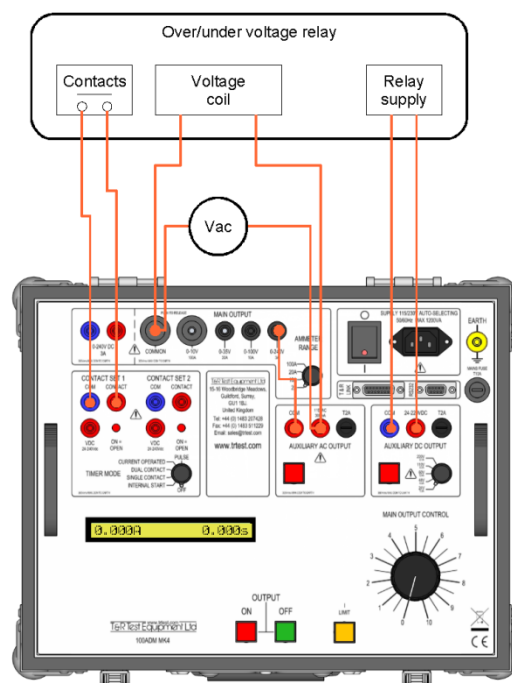
Figure 2.5 Voltage step
