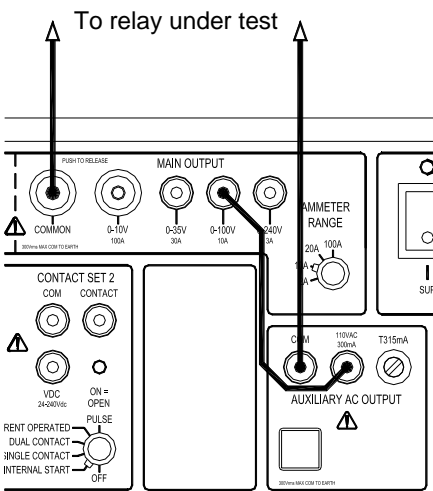
Figure 3.7. Reverse connection – voltage decreases when main output is on.
