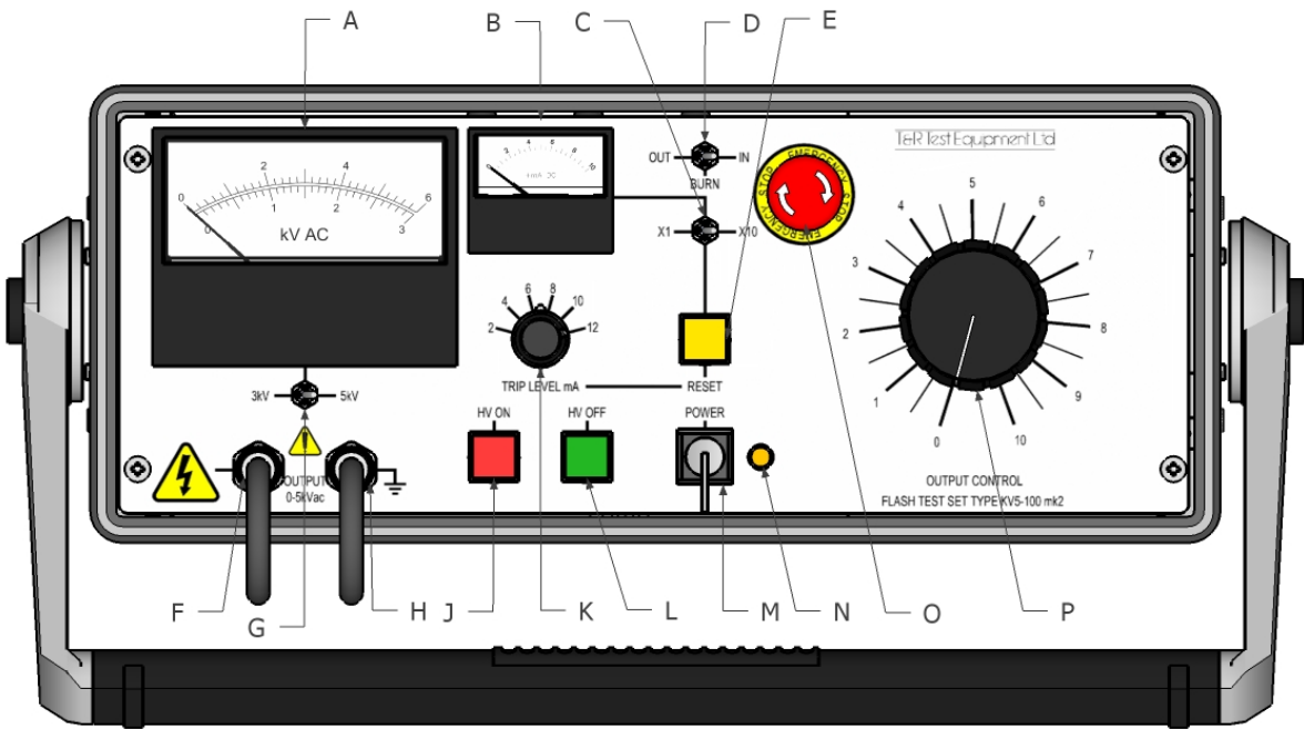
Figure 2.1 KV5-100 mk2 front panel
